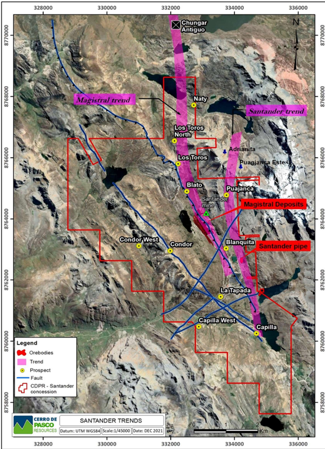
Figure 1: Santander Exploration Targets and known mineral deposits
